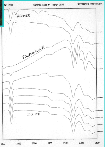
COARSE FELDSPAR PORPHYRY
