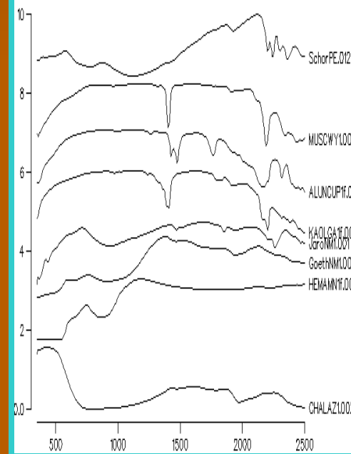
ALTERATION MINERALS TOURMALINE, MUSCOVITE, ALUNITE, KAOLINITE, JAROSITE, GOETHITE, HEMATITE, CHALCANTHITE
