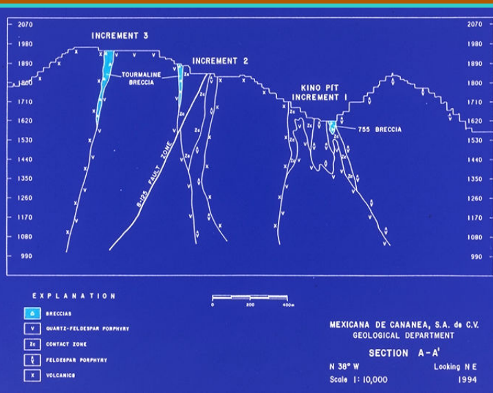
CROSS SECTION SHOWING PITS AND BRECCIAS
